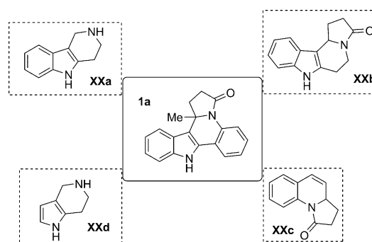
Scheme 4. RCBC product 1a as a hybrid scaffold.
