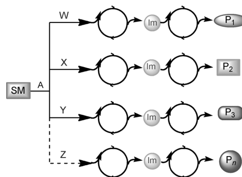
Figure 1. Concept of relay catalytic branching cascade (RCBC).
